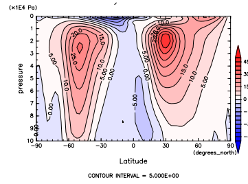
Figure 220: U at Feb. by DCPAM
