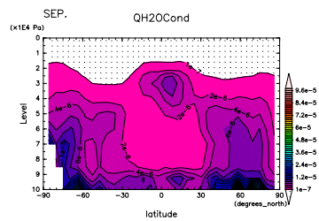
Figure 501: q_l + q_i at Sep. by DCPAM Figure 502: q_l + q_i at Oct. by DCPAM
