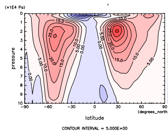
Figure 224: U at Mar. by NCEP
