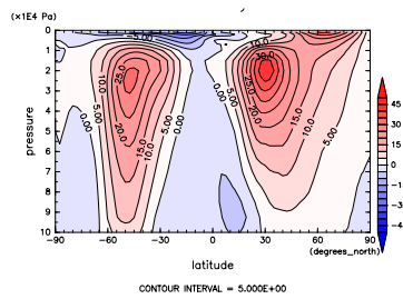
Figure 218: U at Jan. by NCEP
