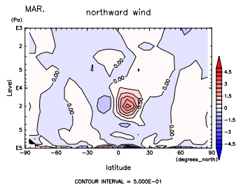
Figure 619: V at Mar. by DCPAM
