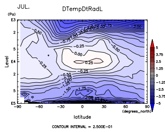
Figure 847: (\partial T / \partial t)_{LW} at Jul. by DCPAM
