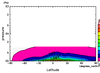
Figure 739: q at Jul. by DCPAM
