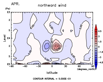
Figure 622: V at Apr. by DCPAM
