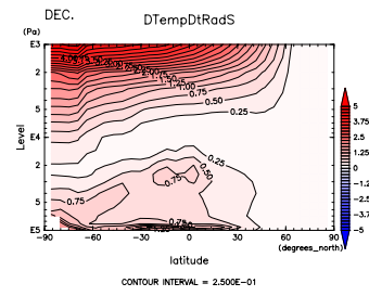
Figure 840: (\partial T/\partial t)_{SW} at Dec. by DCPAM
