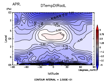
Figure 844: (\partial T / \partial t)_{LW} at Apr. by DCPAM
