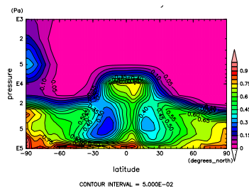
Figure 770: RH at May by NCEP
