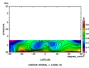
Figure 769: RH at May by DCPAM
