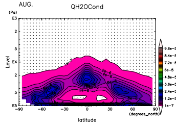
Figure 823: q_l + q_i at Jul. by DCPAM Figure 824: q_l + q_i at Aug. by DCPAM
