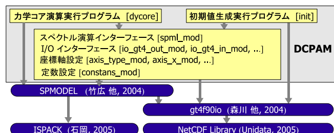
Fig. 1 The structure of DCPAM
