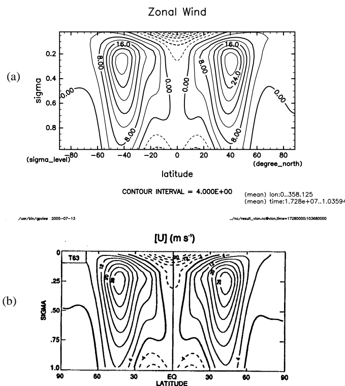
Fig. 7 The zonal-mean zonal wind produced by (a) T63 DCPAM and (b) T63 spectral model of Held and Suarez (from Held and Suarez(1994)). Both are 1000-day means.
