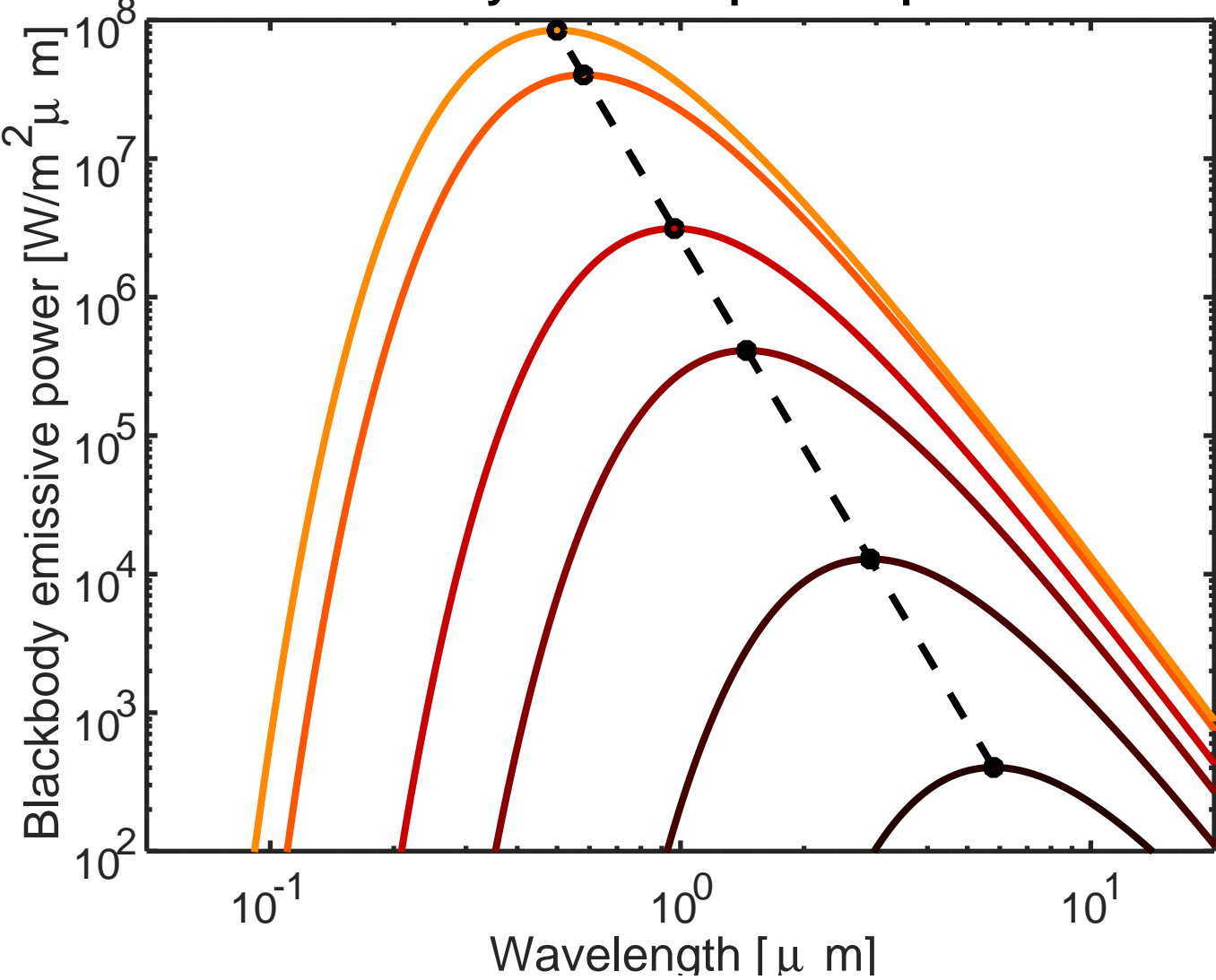
Blackbody emissive power spectrum
