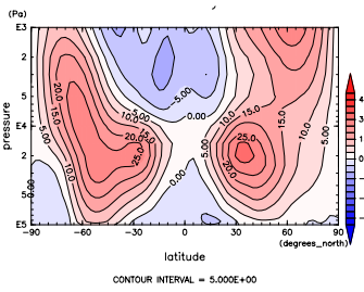
Figure 572: U at Nov. by NCEP
