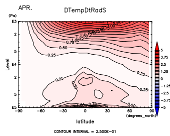
Figure 832: (\partial T/\partial t)_{SW} at Apr. by DCPAM
