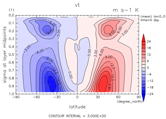
Figure 4: Zonal mean meridional wind and temperature covariance by dcpan
